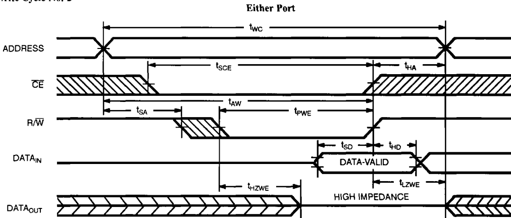
Write Cycle No. 2 [11, 18]
