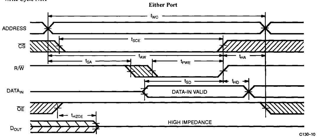
Write Cycle No. 1 [11, 18]
