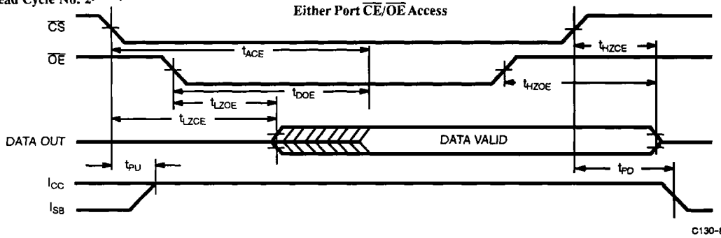
Timing Waveform of Read with \overline{BUSY} [15]
